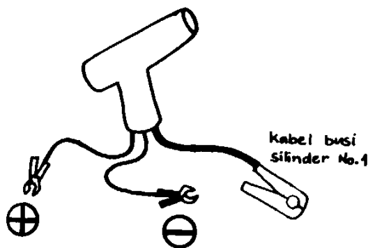
Lampu timing
