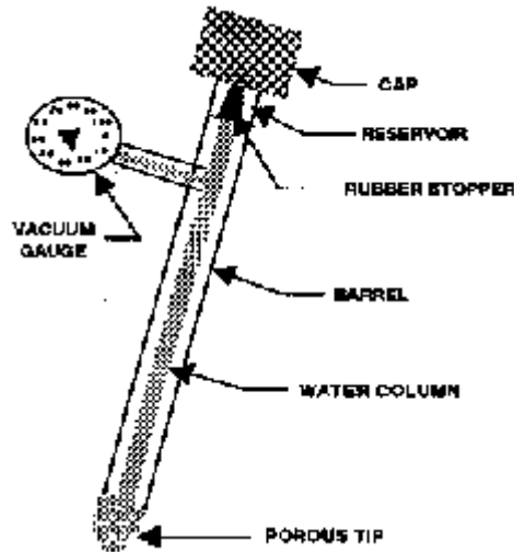
Gambar 31. Tensiometer
