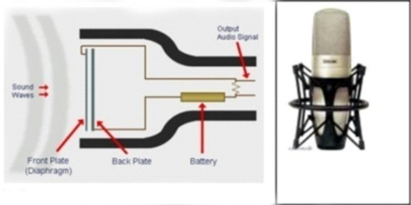
Gambar 229. Condensor microphone
