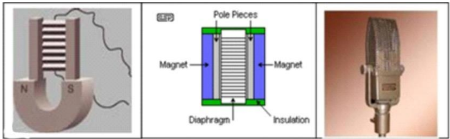
Gambar 231. Ribon microphone
