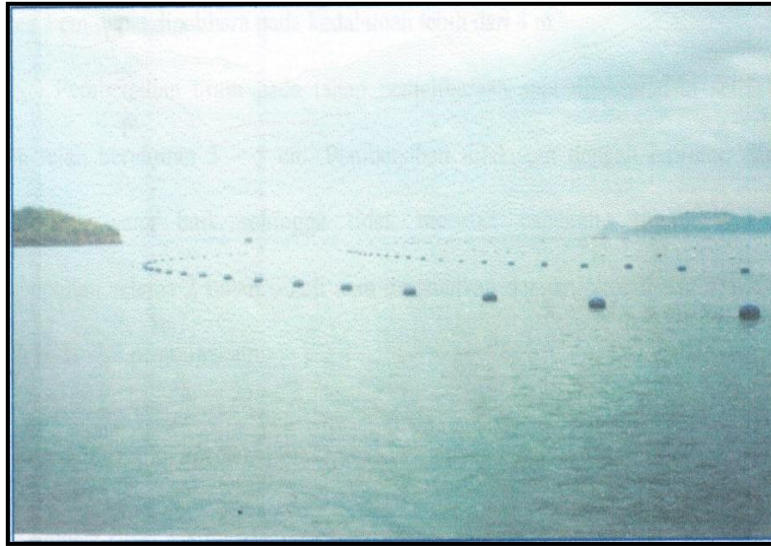
Gambar 13. Sarana budidaya tiram mutiara metode tali rentang ( long line )
