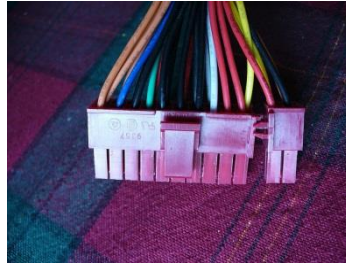
Gambar 57. Konektor 20/24 ATX supply
